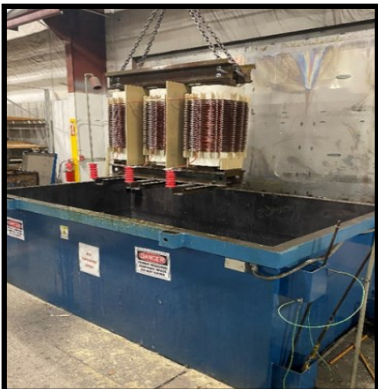
Varnish Dip Process
